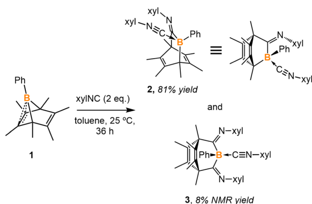
Scheme 1 Reaction of \text{PhB}(\text{C}_6\text{Me}_6) ( 1 ) with 2 equivalents of 2,6-xylyl isocyanide ( \text{xylNC} ) affords 2 in 81% yield and 3 as a side product.
