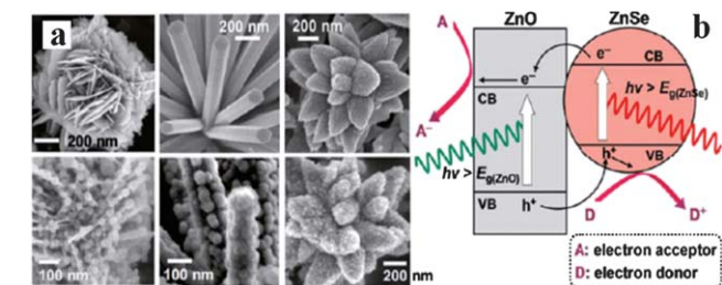
Fig. 11 (a) SEM images of ZnO/ZnSe heterostructures; (b) schematic diagram showing the energy band structures of a ZnO/ZnSe heterostructure (reprinted with permission from ref. 90, copyright 2011 American Chemical Society).
