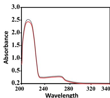
Fig. 2 UV-vis spectra of CuL1 in PBS at 7.4 pH. The solid red and dashed black lines indicate the spectra of fresh solutions and the spectra of solutions after 24 h, respectively.
