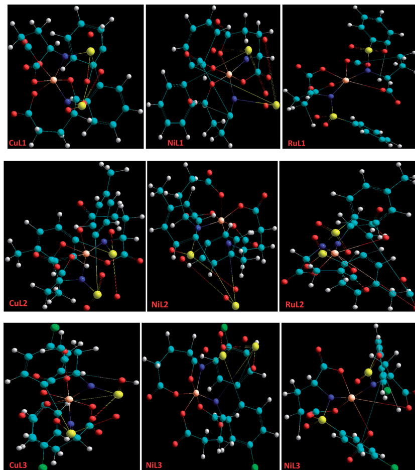
Fig. 3 A perspective view of the ball and stick models of the energy-minimized structures of CuL1 to RuL3 created through molecular modelling. Lone pairs have been excluded for clarity. Nitrogen (blue), sulphur (yellow), carbon (cyan), oxygen (red), chlorine (green), copper, nickel and ruthenium (orange). Sodium cations outside the coordination spheres have been ignored for the energy minimization procedures.
