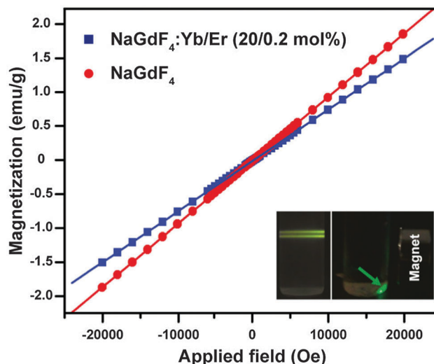
Fig. 24 Magnetization of NaGdF 4 :Yb/Er (20/0.2 mol%) and NaGdF 4 nanocrystals as a function of the applied field. Note that inset shows luminescent photographs of NaGdF 4 :Yb/Er nanocrystals, recorded under excitation at 980 nm, with and without a magnet, indicating that these UC nanocrystals can be recovered by applying an external magnetic force. (Reprinted with permission from ref. 256. Copyright 2011, American Chemical Society.)
