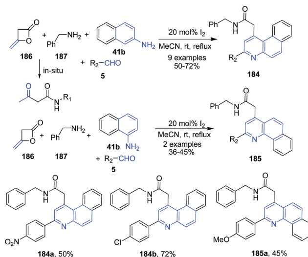
Scheme 65 Molecular iodine catalyzed synthesis of benzo[ f ]quinoliny and benzo[ h ]quinoliny acetamides 184–185 ; some representative examples are shown.
