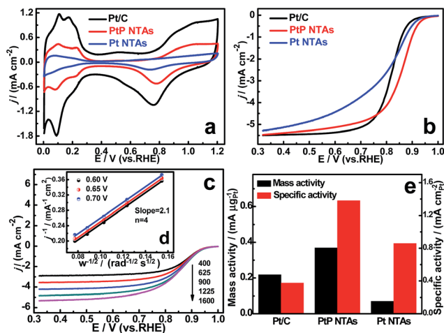
Fig. 3 (a) Cyclic voltammograms for the PtP NTAs, Pt NTAs and Pt/C in N_2 -purged 0.5 M H_2SO_4 at a scan rate of 50 mV\ s^{-1} (Pt loading: \sim 28\ \mu g\ cm^{-2} , S = 0.19625\ cm_{geo}^2 ). (b) ORR polarization curves for the PtP NTAs (40 \mu g\ cm^{-2} ), Pt NTAs (112 \mu g\ cm^{-2} ) and Pt/C (28 \mu g\ cm^{-2} ) in O_2 -saturated 0.1 M HClO_4 with a sweep rate of 5 mV\ s^{-1} and a rotation rate of 1600 rpm. (c) Rotation-rate-dependent current-potential curves for the PtP NTAs (40 \mu g\ cm^{-2} ) in O_2 -saturated 0.1 M HClO_4 . (d) Koutecky-Levich plots for the PtP NTAs at various potentials. (e) Comparison of mass activities and specific activities for the PtP NTAs, Pt NTAs and Pt/C at 0.85 V.
