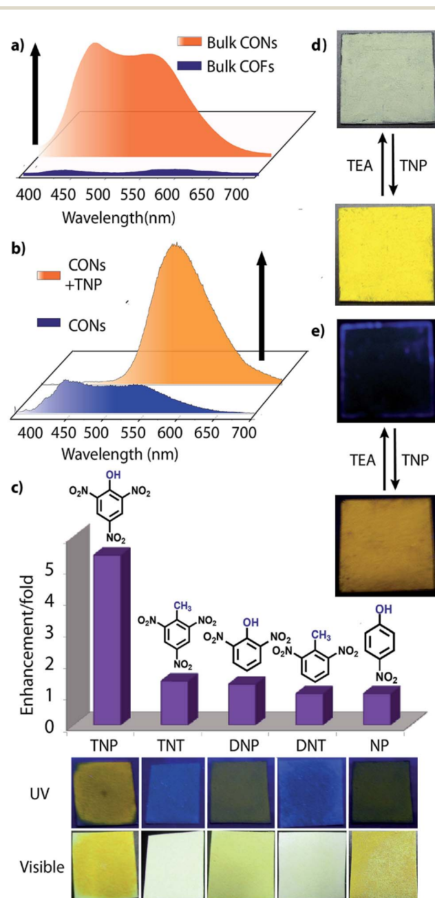
Fig. 6 (a) Photoluminescent spectra of bulk TfpBDH and TfpBDH-CONs ; (b) photoluminescent spectra showing turn on (PL enhancement) of bulk TfpBDH-CONs and with TNP ; (c) photoluminescence enhancement plots of different analytes [at 5.4 \times 10^{-5} (M)] with TfpBDH-CONs ; (d and e) solid state sensing (turn on) by TfpBDH-CONs in presence of TNP under visible and UV light (365 nm) which also exhibits the reversible color change from blue to yellow and vice versa upon TEA treatment.
