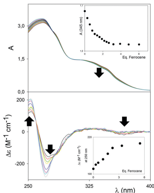
Fig. 2 Top: UV titration of metal-linked macrocycle (RR) - 7 ( 2.5 \times 10^{-5} M) with ferrocene in MeCN at 25^\circ C . Inset: Titration profile vs. ferrocene added equivalents at 345 nm. Bottom: CD titration of macrocycle (RR) - 7 ( 1 \times 10^{-5} M) with ferrocene in MeCN at 25^\circ C . Inset: Titration profile vs. ferrocene added equivalents at 250 nm.
