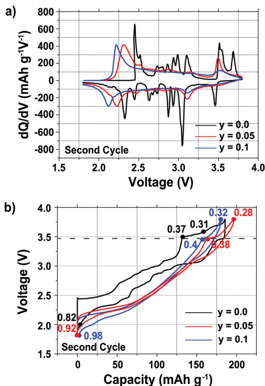
Fig. 1 (a) Differential capacity vs. voltage plots, and (b) electrochemical profiles of the \text{Na}_{2/3}\text{Mn}_{1-y}\text{Mg}_y\text{O}_2 ( y = 0.0, 0.05 and 0.1 ) compositions. The compounds were cycled at 10 \text{ mA g}^{-1} between 1.8 and 3.8 \text{ V} vs. \text{Na}^+/\text{Na} . The electrochemical cells were stopped at different points indicated on the charge/discharge curves to collect the ex situ diffraction data (the numbers on the curves correspond to the Na content, x , at which the cells were stopped). The dotted line at ca. 3.5 \text{ V} indicates the voltage above which a phase transformation occurs in all compositions. The second cycles are shown in order to observe the electrochemical processes occurring below the open circuit voltage (OCV) of the as-synthesized materials, at ca. 2.5 \text{ V} vs. \text{Na}^+/\text{Na} .
