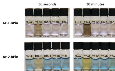
Fig. 3 Photograph of test solutions of Az-1-Bpin and Az-2-Bpin upon exposure to tetra- n -butylammonium halides in THF. In each solution, [analyte] = 180 \mu\text{M} , which for TBAF corresponds to 3.4 \text{mg L}^{-1} of fluoride anion. (For absorption spectra, see Fig. S1 in the ESI†).
