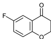
6-fluorobenzo[b]pyran-4-one (51)
