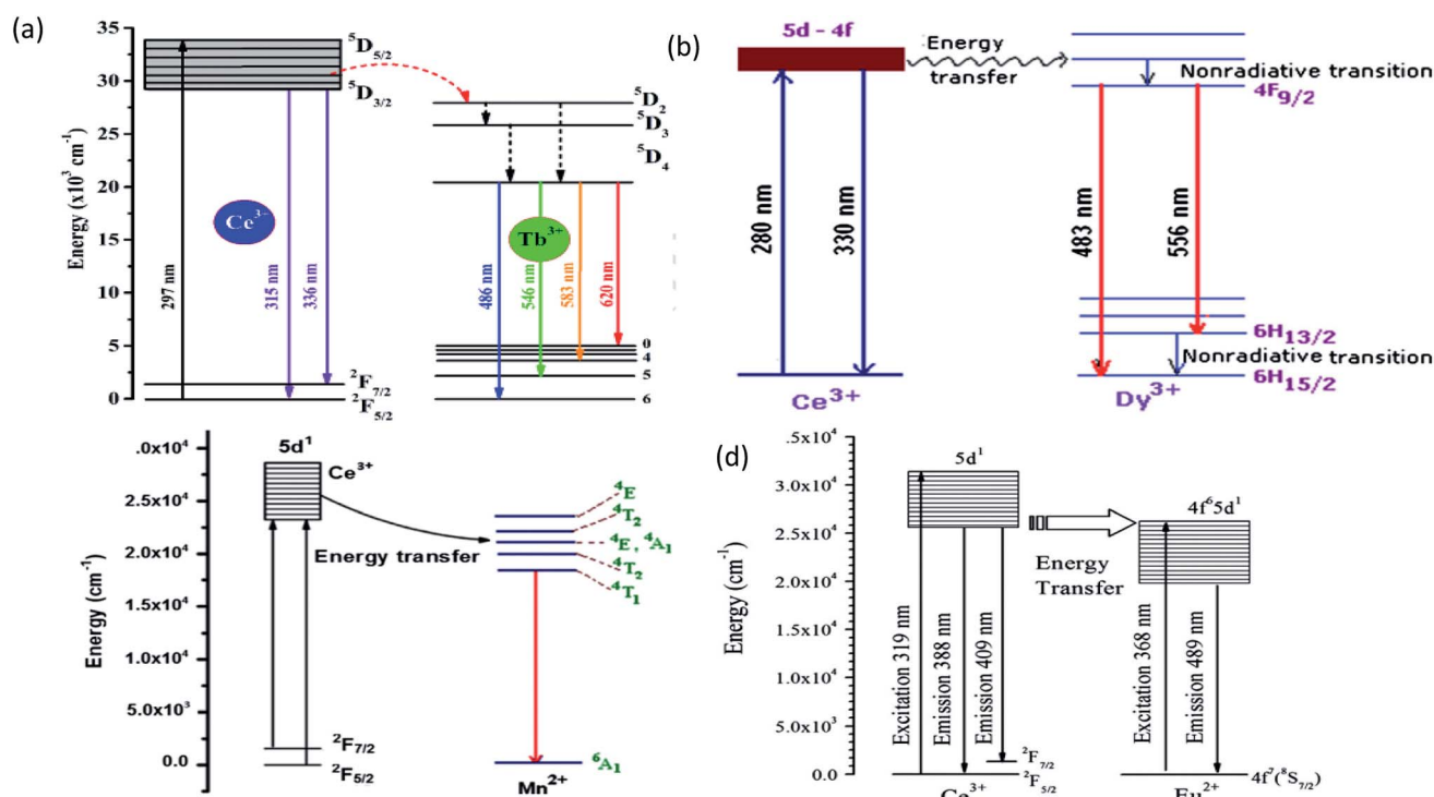
Fig. 14 (a) The schematic energy level diagram for the energy transfer process in the BaMgF 4 :Ce 3+ , Tb 3+ phosphors. 75 (b) Energy level diagram of KNaSO 4 :Ce,Dy. 79 (c) Energy transfer diagram of Ce 3+ → Mn 2+ . 82 (d) Schematic energy-level diagram of Ce 3+ and Eu 2+ . 85
