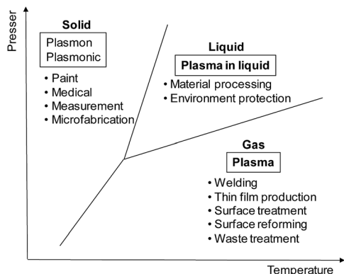
Fig. 2 Relationship between plasma and the three states of matter.
