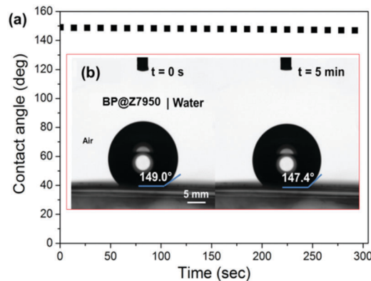
Fig. 4 Contact angle measurements on a PVDF membrane with BP immobilized at the surface. (a) Plot of contact angle (°) over time for a drop of deionized water on the BP supported by PVDF membrane. (b) Optical images (CCD camera) of the contact angle of a deionised water droplet on the BP-coated membrane at t = 0 and 5 min.
