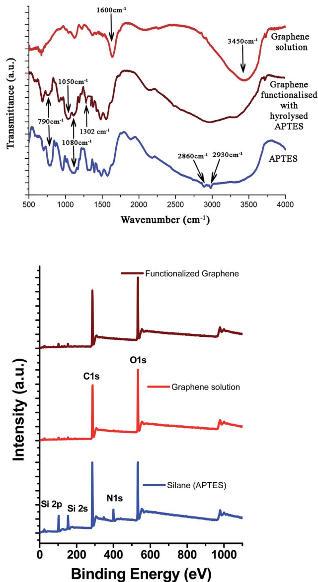
Fig. 4 (a) FTIR spectra of APTES, graphene solution (in water), and graphene functionalized with hydrolyzed APTES. (b) XPS survey spectra of APTES, pure graphene solution, and graphene solution functionalized with APTES.
