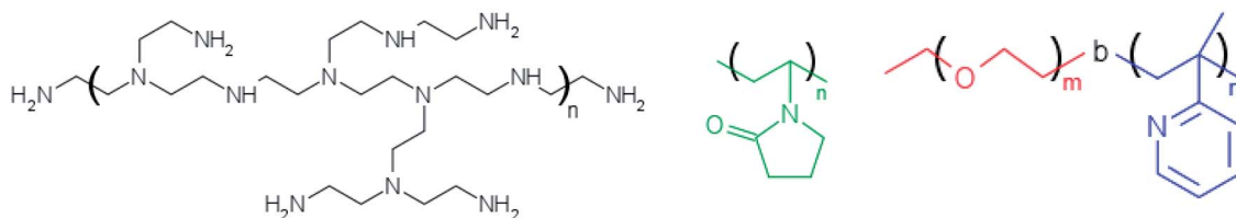
Fig. 1 Molecular structure of branched polyethyleneimine (left), polyvinylpyrrolidone (middle) and poly(ethylene oxide)- b -poly(2-vinyl pyridine) (right).
