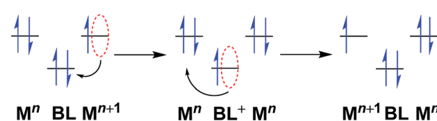
Fig. 4 Bridging ligand-mediated electron transfer and hole transfer pathways in mixed valence complexes. 19c,d
