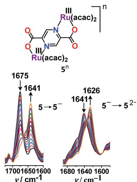
Fig. 6 Shift in the ν(C=O) frequency on moving from 5 → 5 - and 5 - → 5 2- in CH 3 CN.
