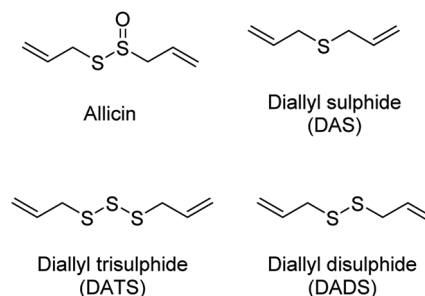
Fig. 3 Naturally occurring \text{H}_2\text{S} donors.
