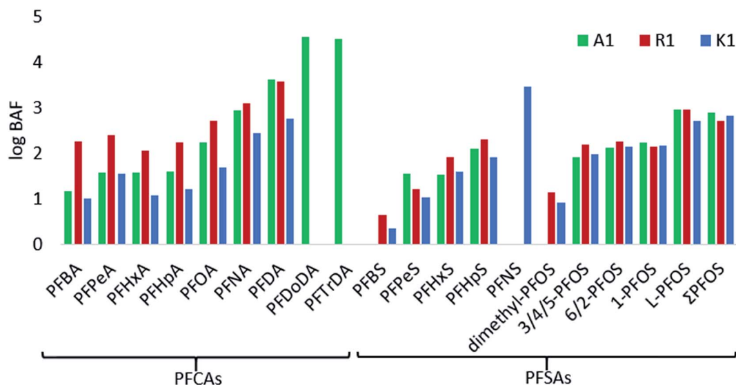
Fig. 4 The logarithmic bioaccumulation factor (BAF) on a wet weight basis ( \text{L kg}^{-1} ) of target PFCAs and PFSA/PFOS isomers (including four branched PFOS isomers, linear PFOS and \Sigma PFOS) for sites A1, R1 and K1. The BAFs could not be determined for some PFASs and sites due to values below MDL.
