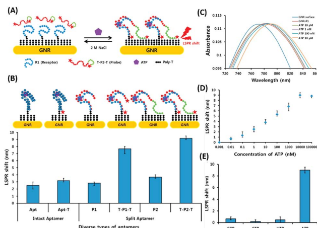
Fig. 10 (A) Schematic representation of the developed LSPR aptasensor for ATP detection based on structure assembly inducing LSPR shift using split-apptamers labelled with TAMRA dye and a random sequence tail. (B) Optimisation of truncation of the aptamer and introduction of TAMRA into the aptamer to achieve maximum LSPR. (C) Shift in LSPR in response to various concentrations of ATP from 10 pM to 10 \mu M. (D) Linear fitting of the LSPR signals for ATP concentrations. (E) Specificity analysis of the developed LSPR based aptasensor for relevant nucleotides. Adapted with permission from ref. 103. Copyright (2015) Elsevier.
