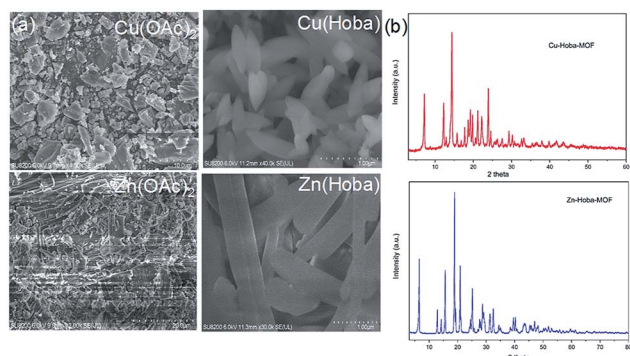
Fig. 1 (a) SEM images of MA precursors (left column) and their respective reaction products with Hobo in water and DMF. (b) PXRD patterns of the products synthesized in one minute.
