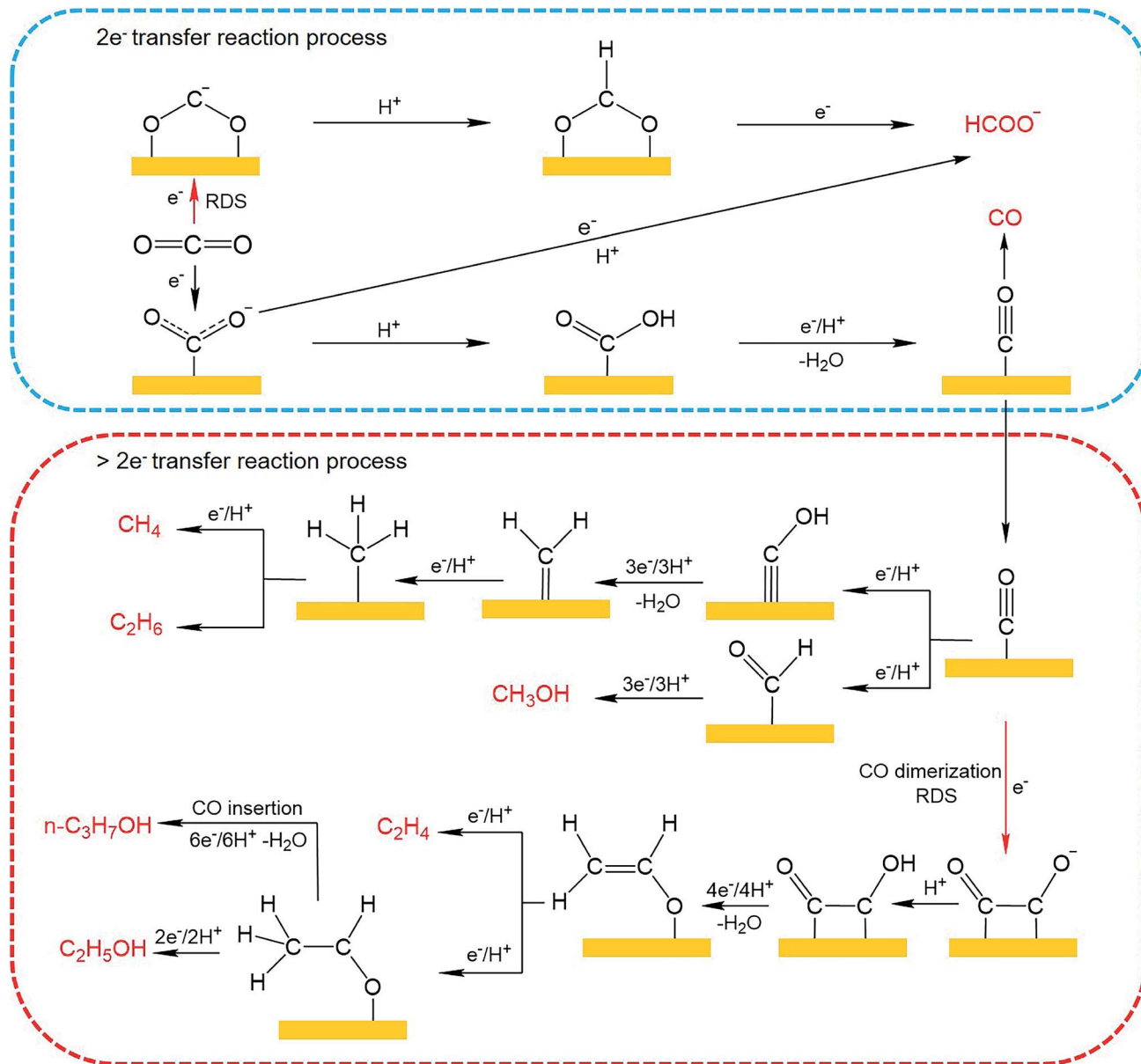
Fig. 9 Possible reaction pathways for \text{CO}_2 electroreduction on Cu-based catalysts toward various products.
