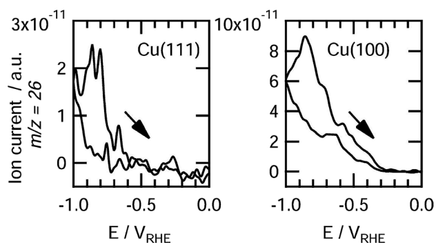
Fig. 10 Detection of ethylene on Cu (111) (left) and Cu (100) (right) during \text{CO} electroreduction by OLEMS. Reprinted from ref. 81 with permission from American Chemical Society.
