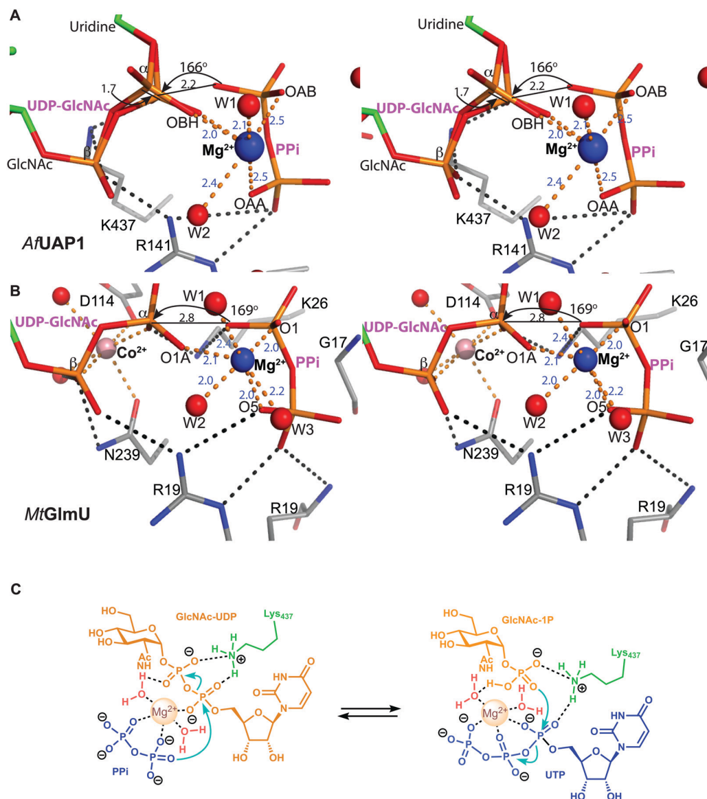
Fig. 5 Magnesium coordination and AfUAP1 mechanism. (A) Magnesium coordination in the AfUAP1 –UDP–GlcNAc–Pi– \text{Mg}^{2+} complex active site. A view of the active site of the AfUAP1 –UDP–GlcNAc–Pi– \text{Mg}^{2+} and MtGlmU –UDP–GlcNAc–Pi– \text{Mg}^{2+} – \text{Co}^{2+} complexes. The attack distance for pyrophosphorolysis is 2.2 and 2.8 Å and the attack angle is 166^\circ and 169^\circ for UAP1 and GlmU, respectively. The distance between the \alpha -phosphates in both UDP–GlcNAc adopting the dual conformation is 1.7 Å. The \text{Mg}^{2+} is tetragonal bipyramidally coordinated (albeit with a disordered 6th ligand in AfUAP1 ) as suggested by coordination distances and angles. (B) Magnesium coordination in the MtGlmU –UDP–GlcNAc–Pi– \text{Mg}^{2+} – \text{Co}^{2+} complex active site. (C) Schematic diagram of the proposed forward and reverse reaction mechanisms. The left panel indicates chemical bond formation/cleavage (cyan arrows) in the AfUAP1 –Pi–UDP–GlcNAc ternary complex shown in Fig. 5A leading to the formation of GlcNAc–1P and UTP. The right panel using the same ternary complex structure as a template indicates chemical bond formation/cleavage in the reverse reaction leading to the formation of UDP–GlcNAc and Pi from GlcNAc–1P and UTP is proposed.
