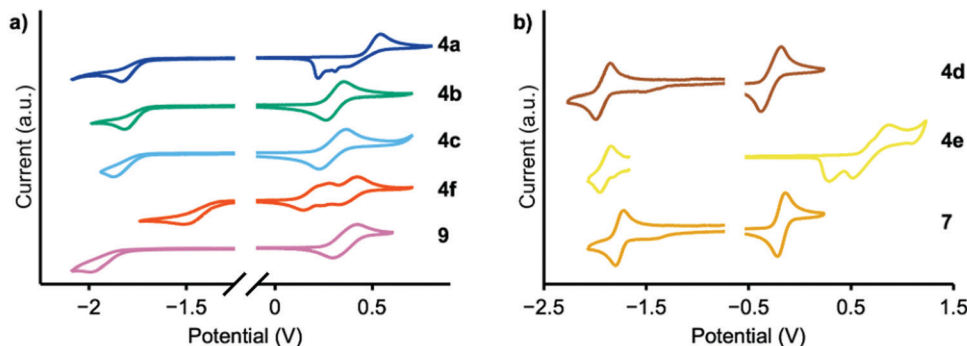
Fig. 4 Cyclic voltammograms of 4a–f , 7 , and 9 relative to \text{Fc}^{0/+} , recorded at a rate of 50 \text{ mV s}^{-1} in THF (a, 4a–c , f , and 9 ) or o-dichlorobenzene (b, 4d , e , and 7 ) containing 0.001 M analyte and 0.2 M tetrabutylammonium hexafluorophosphate as the supporting electrolyte.
