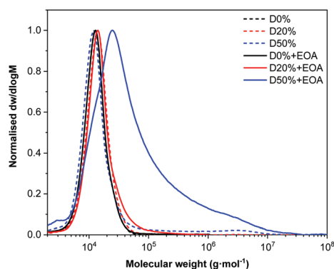
Fig. 4 Normalised SEC RI molecular weight distributions (THF + 2% v/v \text{NEt}_3 , 40^\circ\text{C} , PS standards) of D0%, D20%, and, D50% and before and after treatment with EOA and purification by dialysis.
