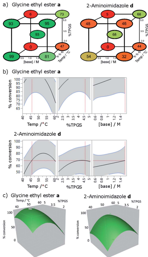
Fig. 3 Optimisation of temperature, surfactant strength (%TPGS) and base concentration by factorial experimental design, conditions: 2 (10 nmol), amine (0.5 M), 2,6-lutidine, DIC (0.5 M), 30 \mu l total volume, 3 h; (a) cube plots showing modelled conversions; (b) % conversion responses for each parameter; (c) response surfaces showing the 2-dimensional effect of temperature and surfactant concentration on conversion. Data shown are fitted using a least squares model ( r^2 = 0.95 , RMSE = 12). For full results see Table S6.†
