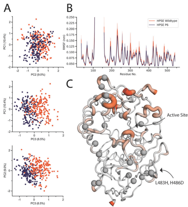
Fig. 4 Molecular dynamic simulations of the wild type the cross design (A) PCA of the two proteins comparing PC1, PC2 and PC3, showing PC3 to have slight differences between the two proteins. (B) RMSF plot of the 95% CI of the wild type, and the mutant average RMSF showing that the mutant stays within the 95% CI, suggesting similar fluctuations. (C) HPSE P6 with average RMSF overlaid. Large RMSF is represented in orange putty, mostly seen around the active site. Mutations are represented as grey spheres.
