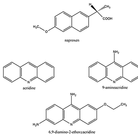
Scheme 1 Molecular structures of naproxen and acridines reported in the paper (the specific chemical forms used are detailed in the Experimental section).
