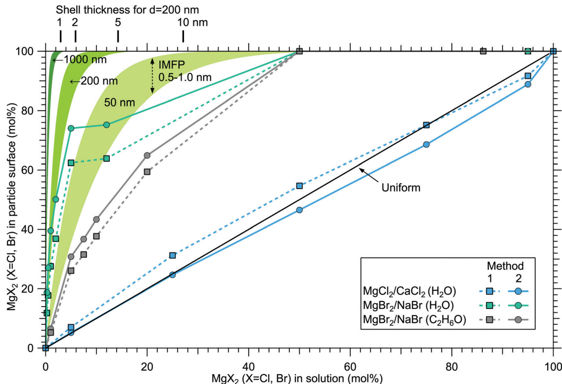
Fig. 8 Surface concentration of \text{MgX}_2 ( X = \text{Cl}, \text{Br} ) plotted as a function of the molar mixing ratio in the atomised solution, obtained as 100 at%/(at%(Mg) + at%(Ca,Na)). For comparison, curves expected from particles with core-shell and uniform structures are shown in green (for diameters 50, 200 and 1000 nm) and black, respectively.
