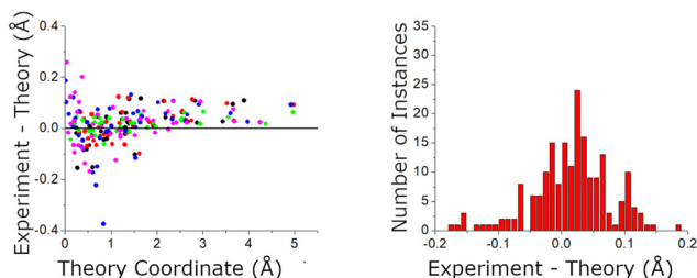
Fig. 9 The accuracy of the quantum chemistry structures is benchmarked using the carbon atom coordinates – in the principal axis system for molecular rotation – obtained from the Kraitzman analysis. The scatter plot shows the difference in the absolute values of these coordinates (coordinate signs are unavailable from the spectroscopic analysis) as a function of the size of the coordinate. The coordinates come from the 5 structures that were measured with ^{13}\text{C} -sensitivity: HOMECD2D1 (black), HOMBC2D1 (blue), HOMBC1D1 (magenta), HETEC1D1 (red), and HETBC1D1 (green). The figure for calculations with the 6-311++G(d,p) basis set is shown in the ESI.†
