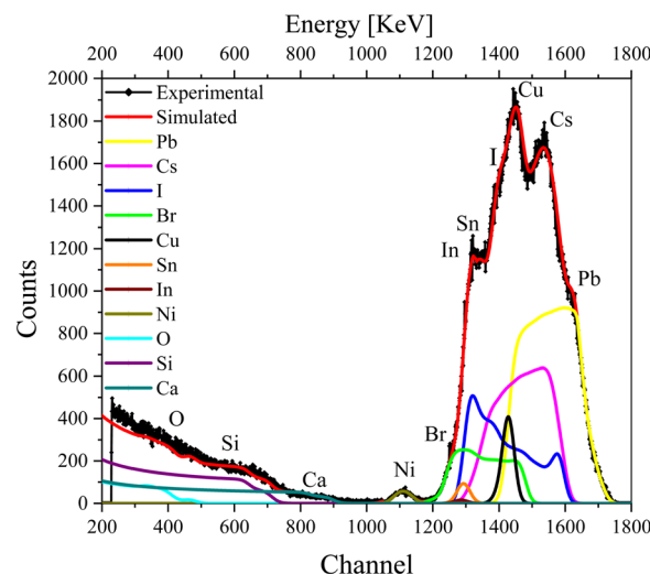
Fig. 4 RBS spectrum of the complete device excited from the Cu contact side, with simulation and deconvolution of the elemental spectra for glass/ITO/ \text{NiO}_x / \text{CsPbI}_2\text{Br} / \text{C}_{60} /Cu.
