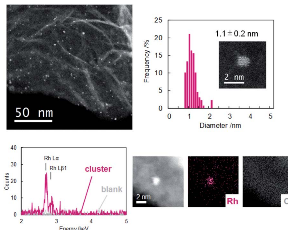
Fig. 2 STEM image, histogram, and EDX analysis of the synthesized Rh nanoparticle.
