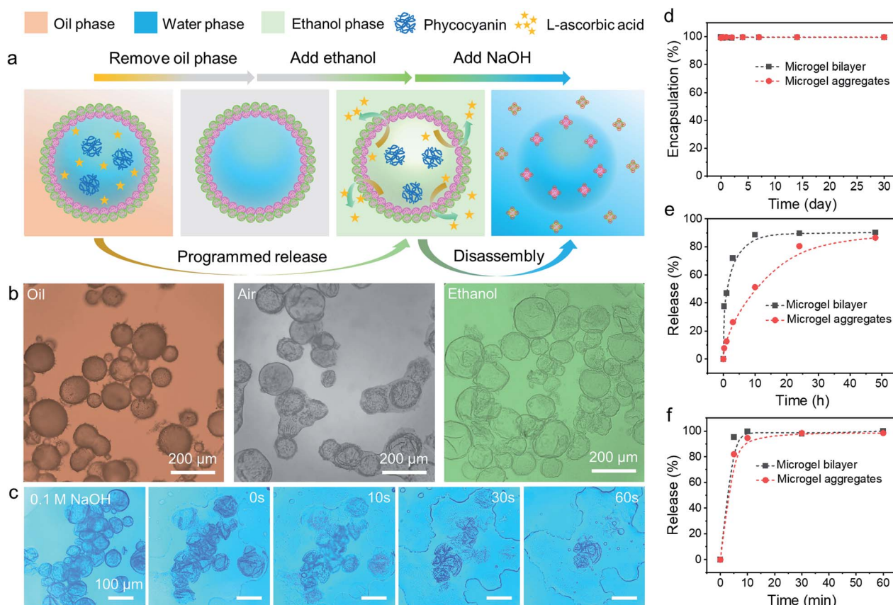
Fig. 6 (a) Schematic illustration of the ethanol induced programmed release and alkali induced disassembly of binary microgel stabilized colloidosomes. (b) Optical microscopy images of the appearance of microgelsomes co-stabilized by PNIPAM- co -MAA microgels and PDEAEMA microgels during the oil removal and ethanol penetration processes. (c) Disassembly of microgelsomes in 0.1 M NaOH. (d) Encapsulation profile of phycocyanin by microgelsomes as a function of time. Programmed release profile of L-ascorbic acid (vitamin C) from microgelsomes (e) in water solution and (f) triggered by additional ethanol.
