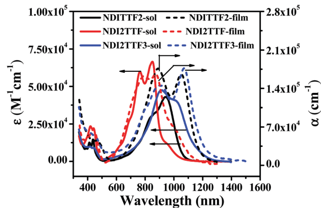
Fig. 1 Absorption spectra of chloroform solutions (solid lines) and thin films (dashed lines) of NDIITTF2 , NDI2TTF and NDI2TTF3 . The concentration for each molecule was 10 μM.
