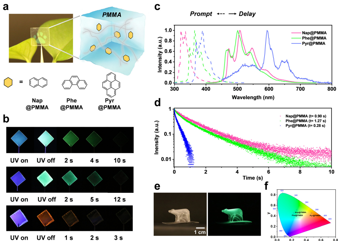
Fig. 1 Ultralong afterglow of PAHs doped in PMMA at room temperature. (a) schematic illustration of the phosphor in rigid polymer surroundings; (b) luminescence photographs under 275 nm UV irradiation and at different time intervals after UV irradiation (from up to down: Nap@PMMA, Phe@PMMA, and Pyr@PMMA); (c) steady-state fluorescence and delayed RTP spectra (delay time: 10 ms); (d) time-resolved RTP decay curves of Nap@PMMA at 508 nm, Phe@PMMA at 500 nm and Pyr@PMMA at 596 nm ( \lambda_{\text{ex}} = 275 nm); (e) transparent 3D bear of Nap@PMMA showing long-lived RTP; (f) CIE coordinate diagrams of Nap@PMMA, Phe@PMMA, and Pyr@PMMA.
