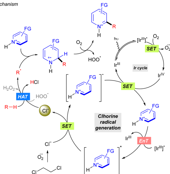
Scheme 13 Minisci-type alkylation through dual iridium/ \text{Cl}^* catalysis.
