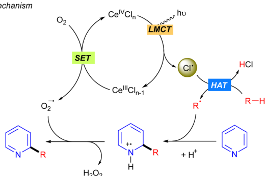
Scheme 12 Minisci-type alkylation through dual cerium/ \text{Cl}^* catalysis.
