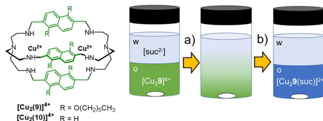
Fig. 9 Schematized structures of the dicopper cryptates of cages 9 and 10, and application of [\text{Cu}_2(9)]^{4+} as extractant for succinate 76 from aqueous solutions ( 0.05 \text{ mol L}^{-1} HEPES buffer, pH = 7) into dichloromethane. The transfer of succinate into the organic phase and its binding into the cryptate cavity are accompanied by a change of colour in the organic phase, from green to blue.
