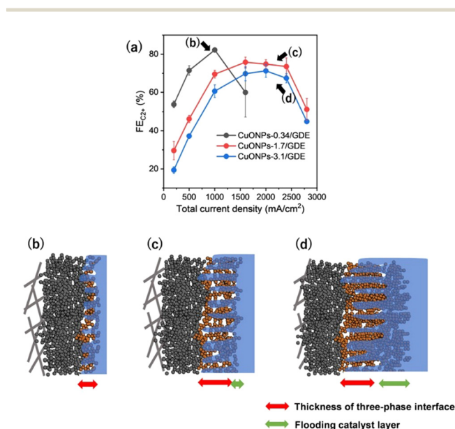
Fig. 4 (a) FE C 2+ against J_{\text{total}} for various amounts of Cu loading (CuONPs-0.34, -1.7 and -3.1/GDE) in 1 M KCl. (b–d) Schematic image of the three-phase interfaces at each position which are indicated in (a). The red and green arrows represent the thickness of three-phase interface and flooding catalyst layer, respectively.
