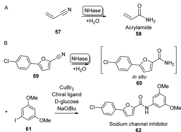
Scheme 11 Nitrile Hydratase (NHase) catalysed amide bond formation. (A) NHase catalysed acrylamide synthesis. (B) Chemoenzymatic strategy for the expansion of amide scopes using copper catalysis. 87
