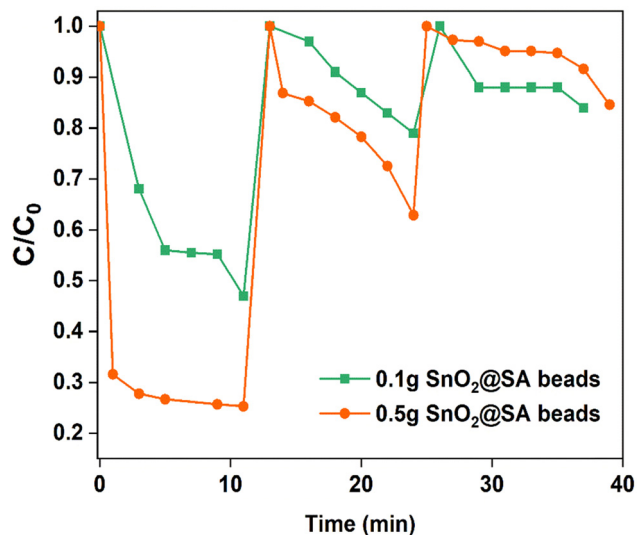
Fig. 12 Regenerative studies of 0.5 g and 0.1 g \text{SnO}_2 @SA beads for 5 \mu\text{M} CR aqueous solution.
