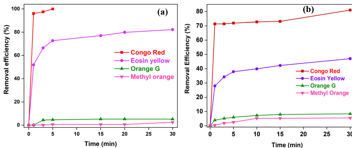
Fig. 5 Adsorption of four anionic dyes at a concentration of 5 \mu\text{M} using (a) 0.1 g/100 mL of \text{SnO}_2 NPs and (b) 0.3 g \text{SnO}_2 @SA beads.
