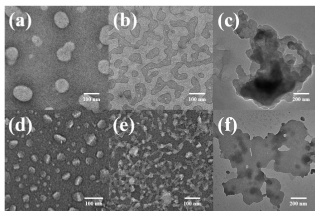
Fig. 9 TEM images of molecule H 1 C G ( c/c = 4:1 ) obtained from \text{CHCl}_3/\text{DMSO} ( v/v = 19:1 ) solutions after (a) 1 h, (b) 4 h and (c) 24 h. TEM images of molecule H 2 C G ( c/c = 4:1 ) obtained from \text{CHCl}_3/\text{DMSO} ( v/v = 19:1 ) solution after (d) 1 h, (e) 4 h and (f) 24 h.
