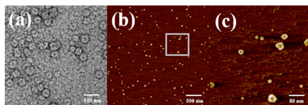
Fig. 6 (a) Negative-staining TEM images and (b) AFM images of cis - H 1 ( H 1 after irradiation with 365 nm UV light for 20 min) obtained from 3.03 \times 10^{-6} mol L -1 H 2 O/DMSO (v/v = 19 : 1) solutions. (c) Enlarged image of part b.
