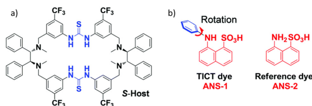
Fig. 12 Chemical structures of the chiral host (a), and the achiral fluorescent guest (b). Adopted with permission from ref. 142. Copyright 2020, Royal Society of Chemistry.
