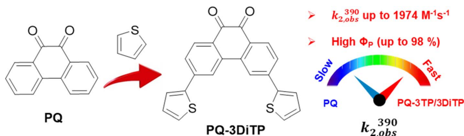
Scheme 1 Comparison of photocycloaddition of 9,10-phenanthrenequinone ( PQ ) with electron-rich alkenes ( ERAs ). k_{2,\text{obs}}(390) observed second-order reaction rate; and \Phi_{\text{P}} : photoreaction quantum yield.
