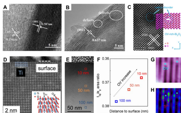
Fig. 2 HRTEM images of (A) pristine SnS 2 and (B) SnS 2 featuring Al doping 43 copyright © 2021 Elsevier B.V. (C) HAADF-STEM images of VO-rich-Bi 2 O 3 nanosheets, the scale bar is 2 nm. 45 Copyright © 2019, Springer Nature Limited. STEM image of cross-sectional TiO 2 (110) single crystal (D) and large region (E). (F) Concentration of O vacancies increased from inner to surface regions. (G) STM image of the TiO 2 surface in the empty state. (H) STM image of the same region of (G), but in the filled state 46 copyright © 2018 American Chemical Society.
