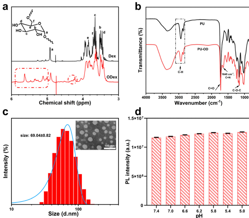
Fig. 1 (a) 1 H NMR spectra of dextran and oxidized dextran. (b) FTIR spectra of PU and PU-OD hydrogel. (c) Diagram of particle size distribution of PU emulsion and the TEM image of PU. (d) Maximum value of the fluorescence emission intensity of PU emulsion (200 μg mL -1 ) at different pH ( n , repeated value, n = 3).
