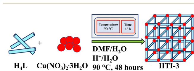
Scheme 1 Schematic synthesis of IITI-3.
