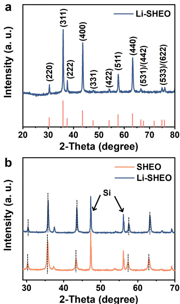
Fig. 1 XRD patterns of (a) Li-SHEO material, and (b) SHEO and Li-SHEO materials for revealing the peak shift behaviour.
