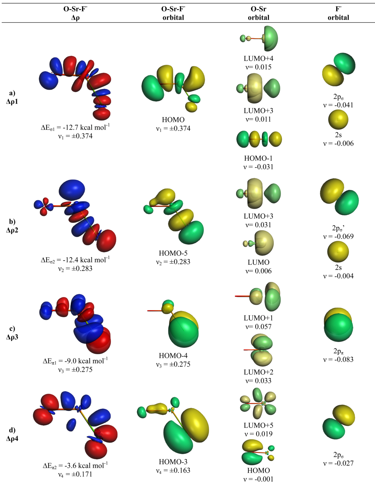
Fig. 8 Plot of deformation densities \Delta\rho of \text{OSrF}^- . The pairwise orbital interactions and the associated interaction energies ( \Delta E_{\text{orb}} ) between fragments OSr (S) and F - (S) in \text{OSrF}^- at the equilibrium structure, as well as the shape of the most important interacting MOs. The direction of the charge flow is red \rightarrow blue. (Isovalue 0.03e a.u. -3 ).
