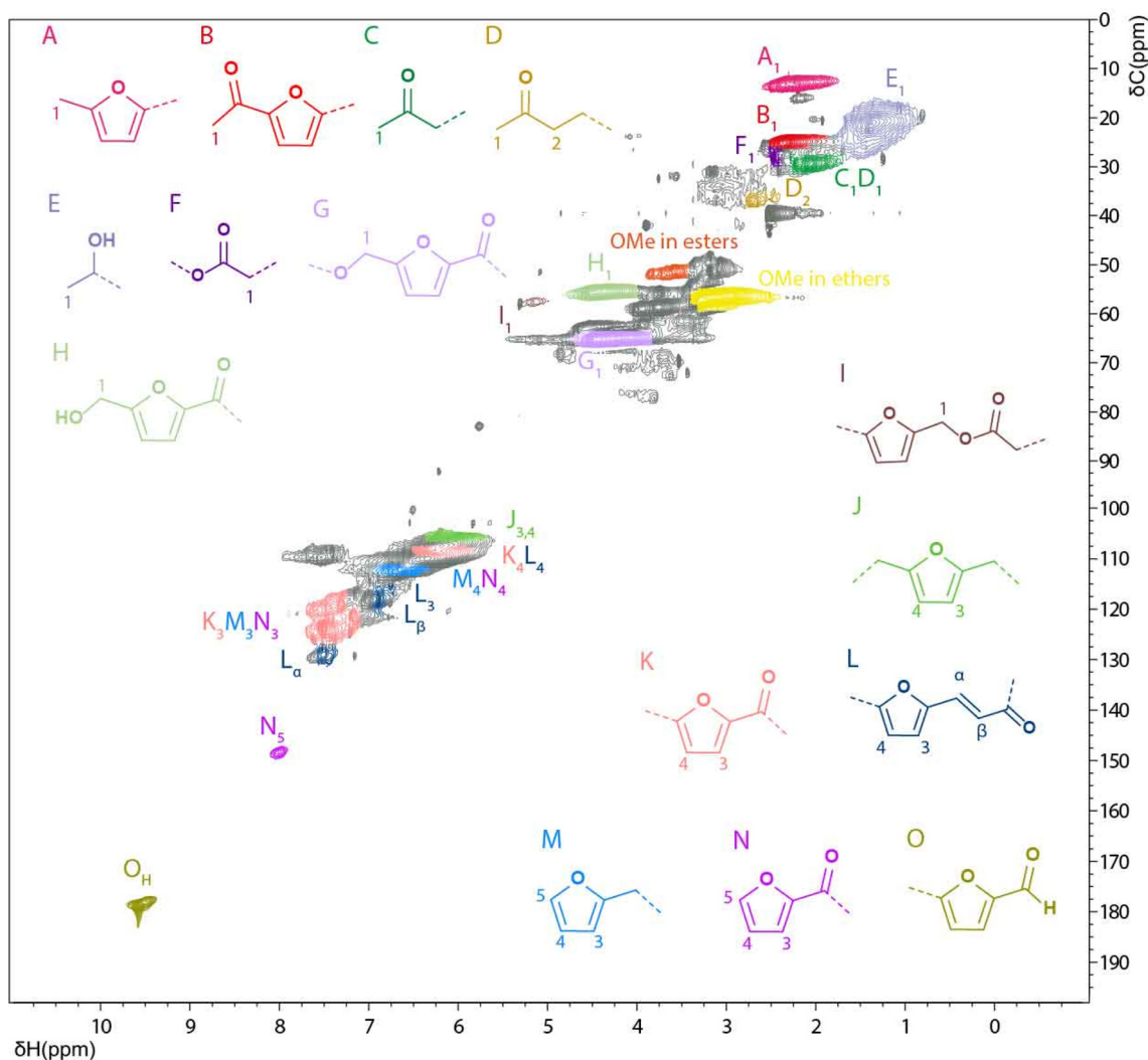
Fig. 5 Solution state [ ^1H ; ^{13}C ] HSQC NMR spectrum of the WIPIH fraction in DMSO- d_6 and main structural motifs identified.
