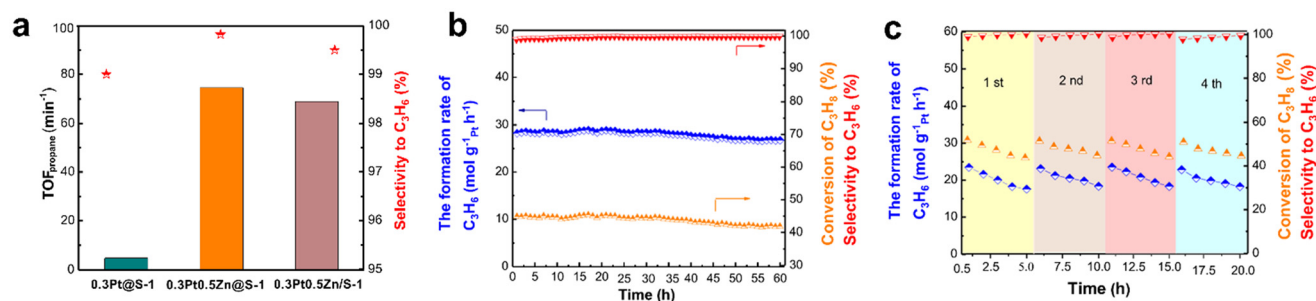
Fig. 19 (a) The TOF of Pt-based catalysts at 450 °C; (b) stability testing over 0.3Pt0.5Zn@S-1 at 550 °C for 60 h; (c) recyclability of 0.3Pt0.5Zn@S-1 in the PDH reaction at 600 °C (reaction conditions: 200 mg catalysts, atmospheric pressure, \text{WHSV}_{\text{propane}} = 6.5\text{ h}^{-1} , and \text{C}_3\text{H}_8:\text{N}_2 = 11:19 with flow rate 30\text{ mL min}^{-1} ). 136 Reprinted with permission from Elsevier Inc., copyright 2020.
